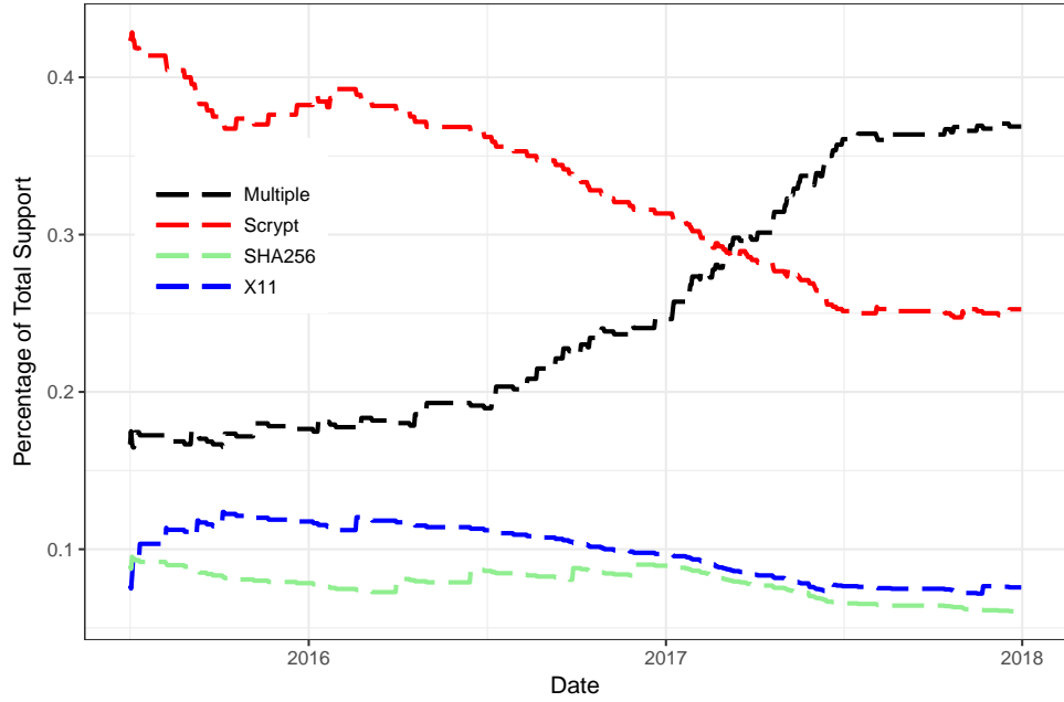
(a) Algorithm
