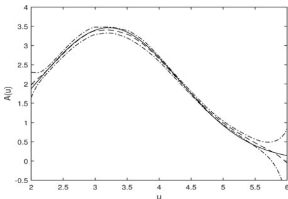
Figure 1. The estimated A(u) when the sample size n = 500 . The solid line represents the true A(u) , and the dashed line denotes the estimated values. The two dash-dotted lines are the 90% pointwise confidence intervals with bias ignored.
