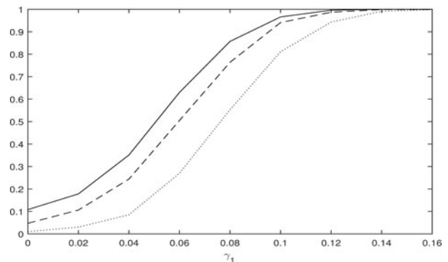
Figure 3. The power curves of testing H_0 : \beta_1 = -1, \beta_2 = 1 against H_1 : \beta_1 = -1 + \gamma_1, \beta_2 = 1 for sample size n = 500 . The dotted line is the power curve for 1% significance level, the dashed line and the solid line are for 5% and 10% significance levels, respectively.
