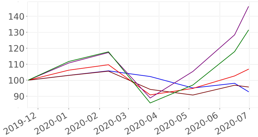
Figure 13: Backtesting on EM FIs data: classical approaches ( MinVar , IVP , HRP ) vs uplifted approaches ( Inv \lambda , upHRP )
