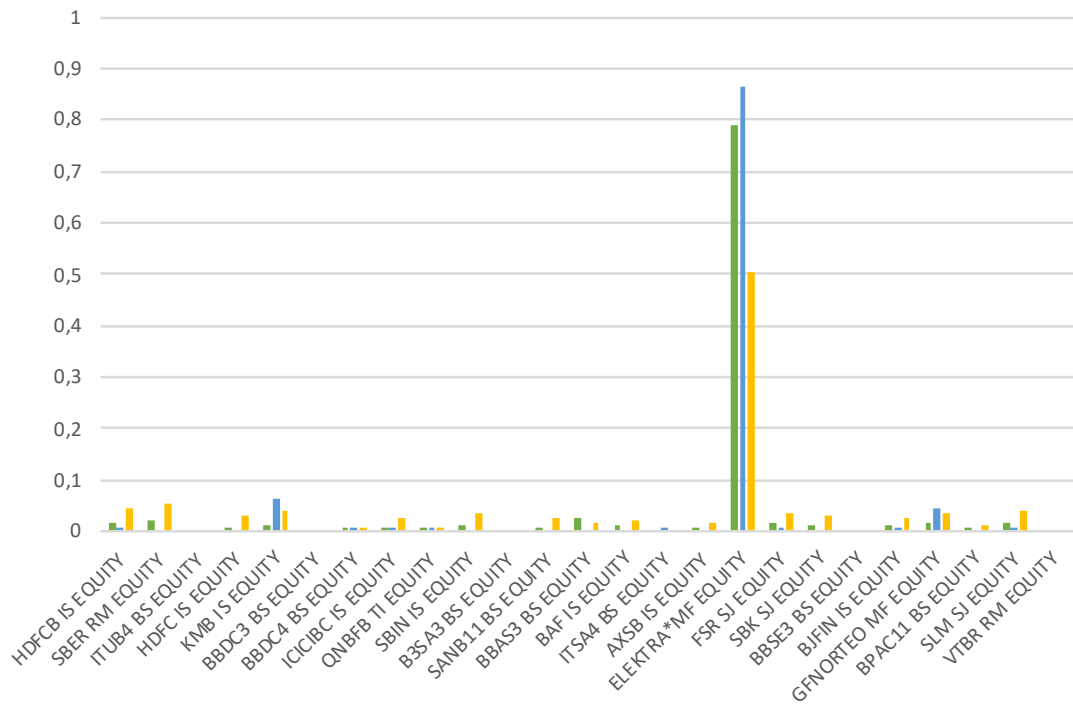
(a) Optimal weights MinVar, IVP, HRP
