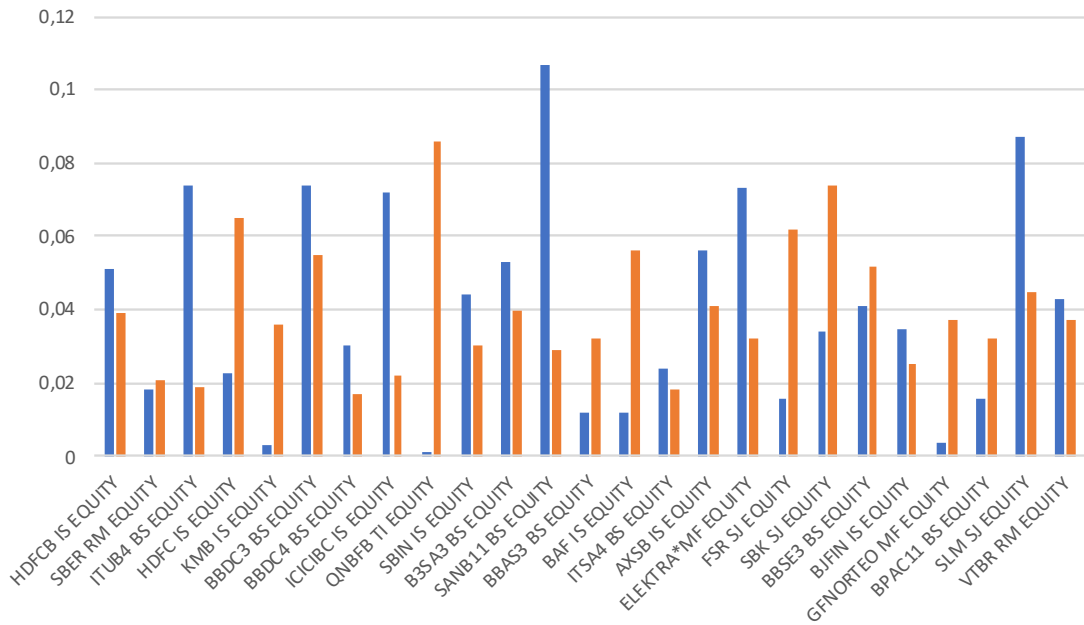
(b) Optimal weights Invλ, upHRP
