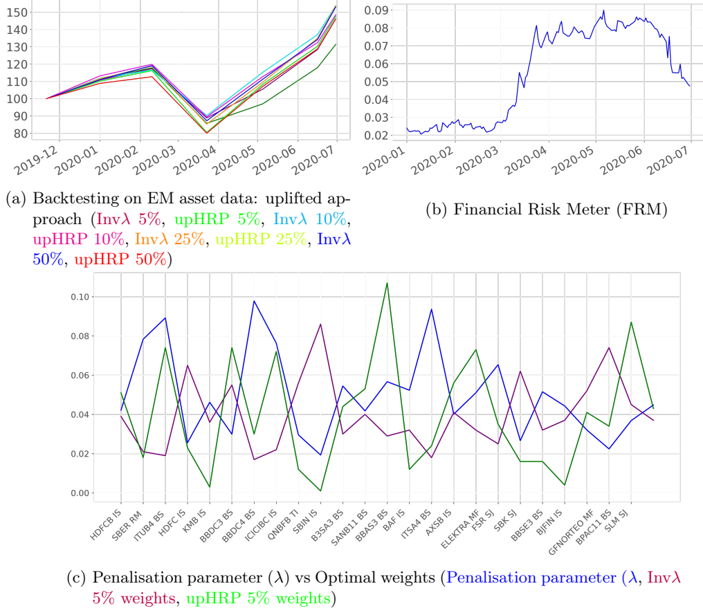
Figure 14: Impact of Penalisation parameter ( \lambda ) and FRM on optimal weights and portfolio returns
