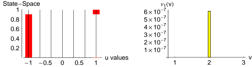
FIG 2. Optimal Absolutely Continuous and Singular Control Policies in Regime y = 1 .
