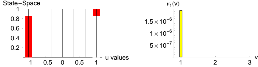
FIG 1. Optimal Absolutely Continuous and Singular Control Policies in Regime y = 0 .
