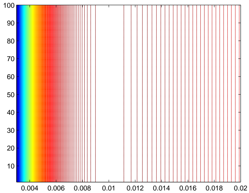
(b) Likelihood
