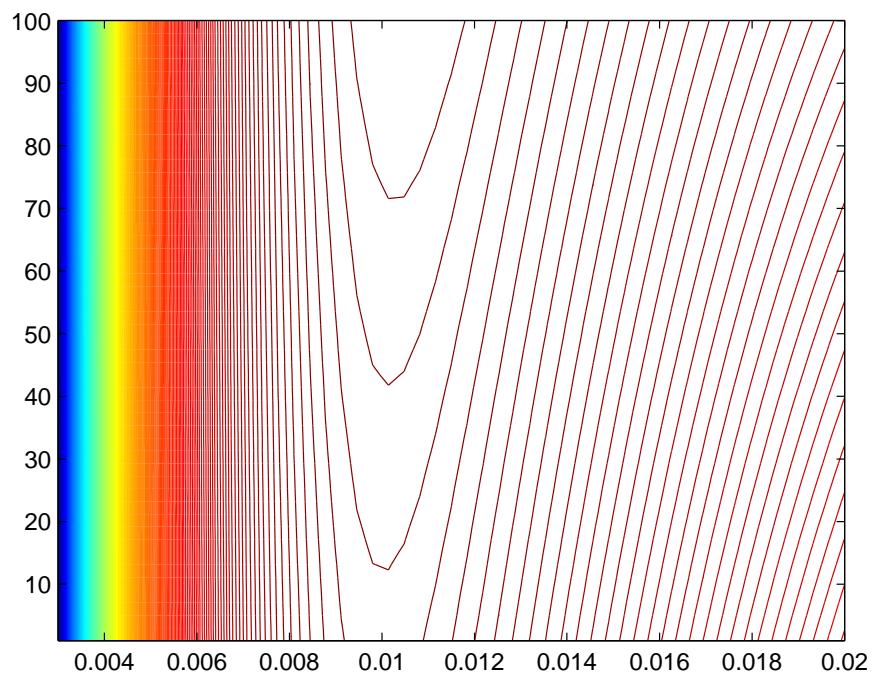
(b) Likelihood
