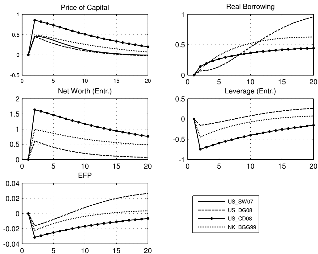
Figure 8: IRFs to a Positive Technology Shock under SW Rule: Financial Variables
