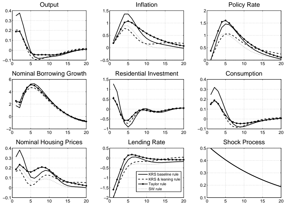
Figure 16: IRFs to a financial shock reducing the interest rate spread
