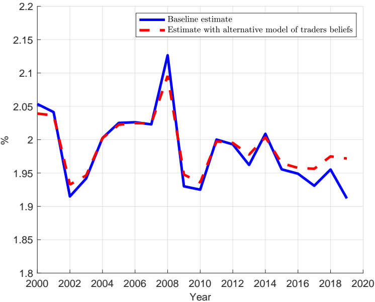
Figure A2: Excess weight statistic
