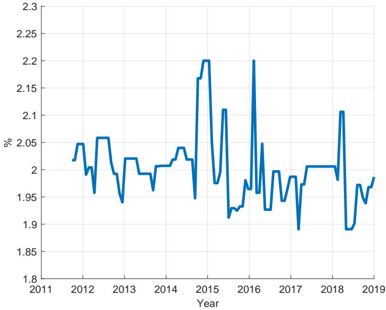
Figure A6: The expected percentile of the marginal trader since 2000
